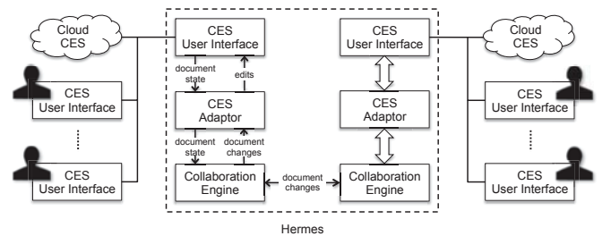
Fig. 2. Hermes architecture.
